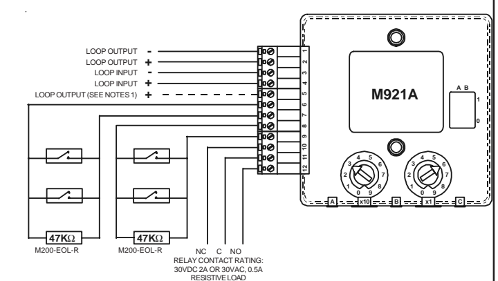
FIGURE 4: M921A DUAL INPUT SINGLE OUTPUT MODULE WIRING
