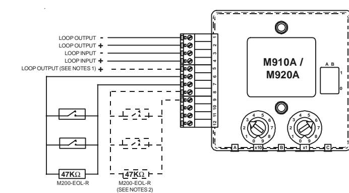
FIGURE 3: M910A SINGLE INPUT AND M920A DUAL INPUT MODULE WIRING
