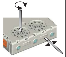
FIGURE 2: ROTARY DECADE ADDRESS SWITCHES
