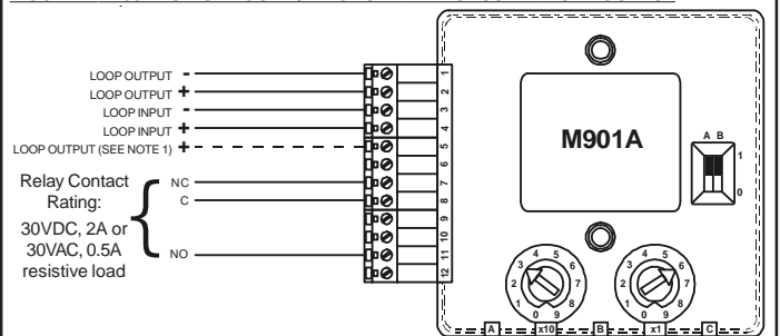
FIGURE 4: M901A SINGLE OUTPUT MODULE WITH UNSUPERVISED OUTPUT
