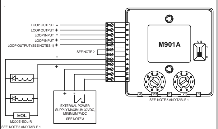
FIGURE 3: M901A SINGLE OUTPUT MODULE WITH SUPERVISED OUTPUT
